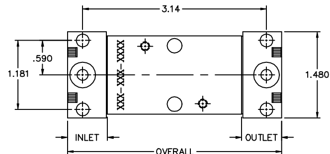
OPTIONAL DOWNPORT FITTING
